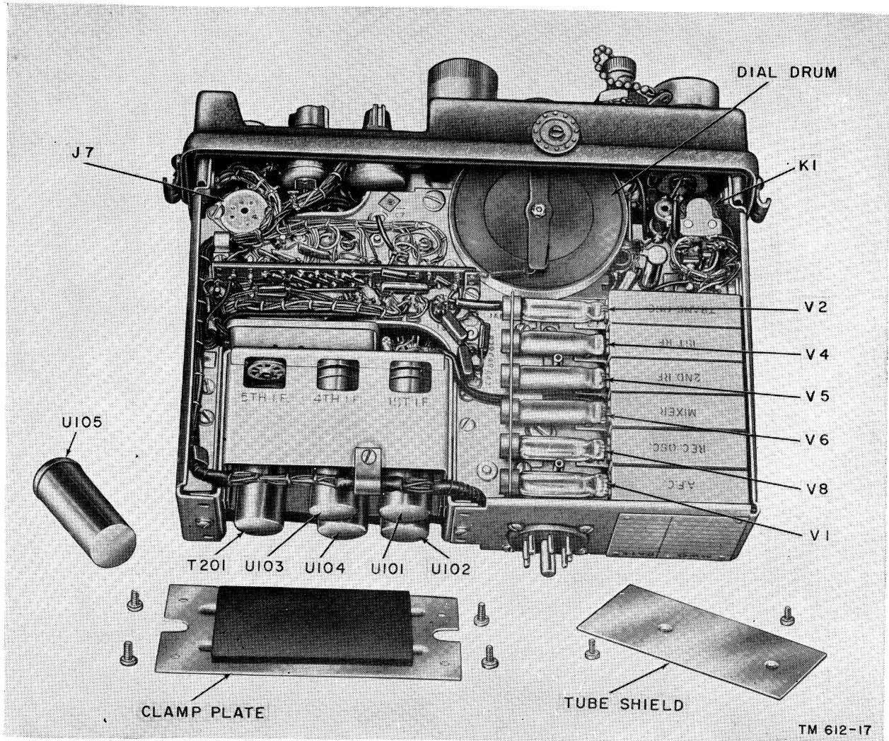
Figure 27. Receiver-transmitter chassis (unlettered models), top view.
